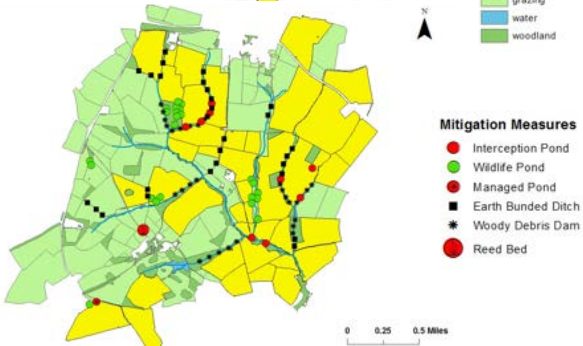
Figure 50. Locations of mitigation measures in (a) Eye Brook and (b) Stonton Brook catchments. Measures are mainly concentrated in the arable farmed environment.
