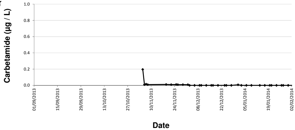
Figure 48. Carbetamide runoff in winter 2013/14. (a) Barkby Brook (b) Eye Brook (c) Stonton Brook.
